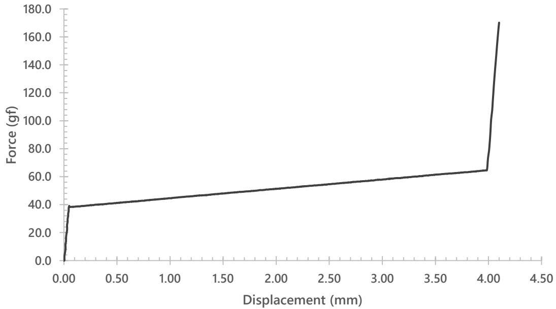
Varmilo Rose Capacitive V3 (Upstroke)
